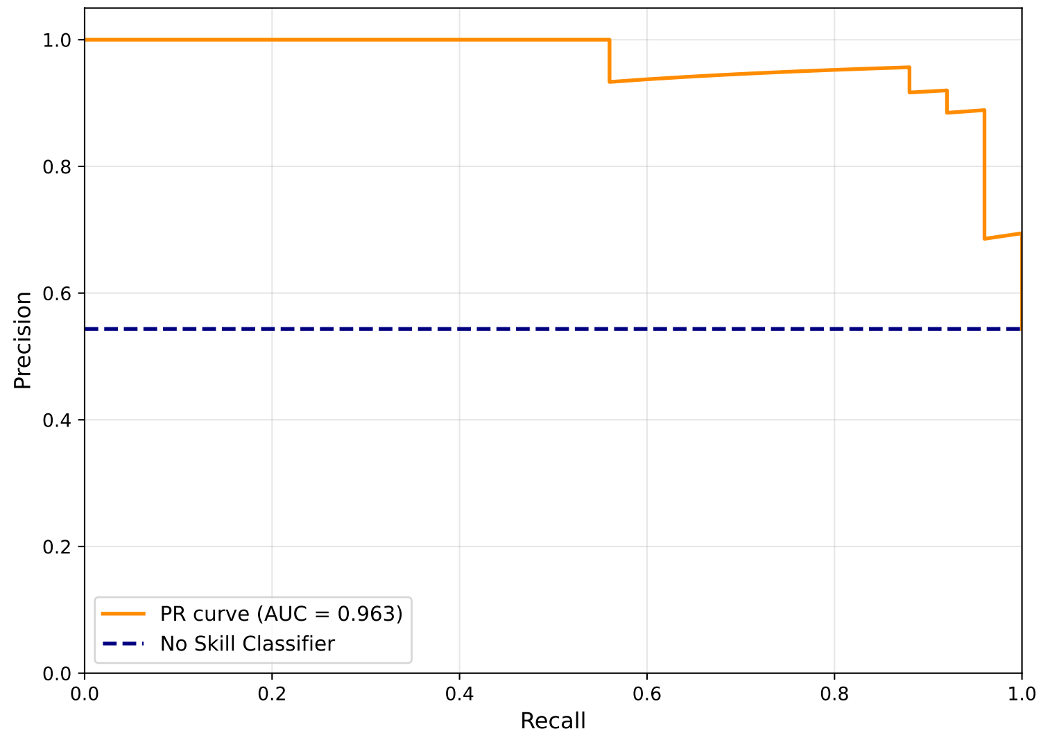
Precision-Recall Curve for Tuned Random Forest
